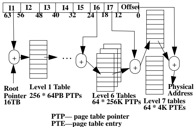
Figure 3: Forward-mapped page table
